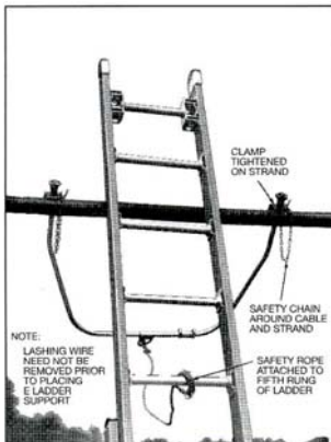
E Ladder Support in position on strand
