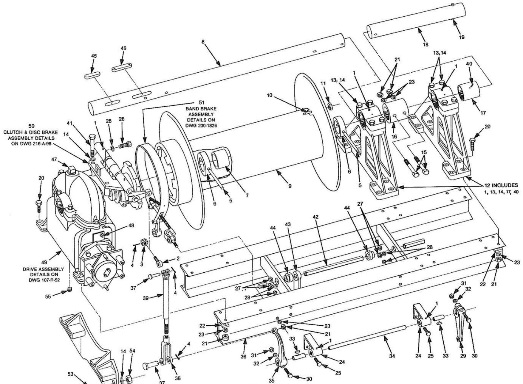
FIG. 2 GENERAL ASSEMBLY PARTS DRAWING
