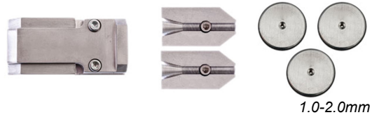
Cable Seal Collet Assemblies
