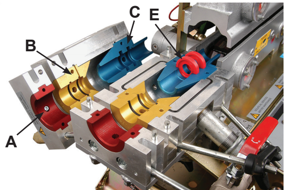
EXIT SIDE
