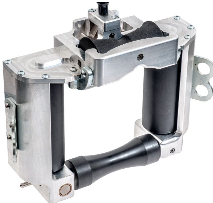
ASSEMBLY FRONT LIFTER - SUPER G LASHER p/n 37295
