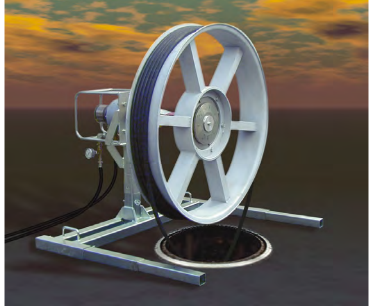
Hydraulically Limited Cable Puller with Mid-Assist Fiber Optic Capstan
